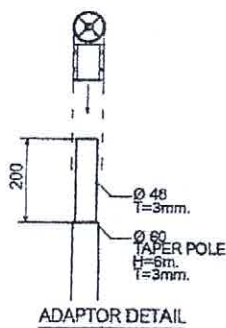
ADAPTOR DETAIL
